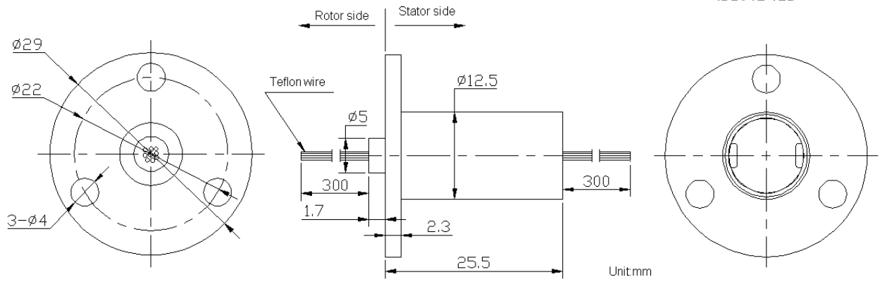
MODEL:BLC12-12B
