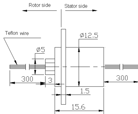
MODEL:BLC12-04A
