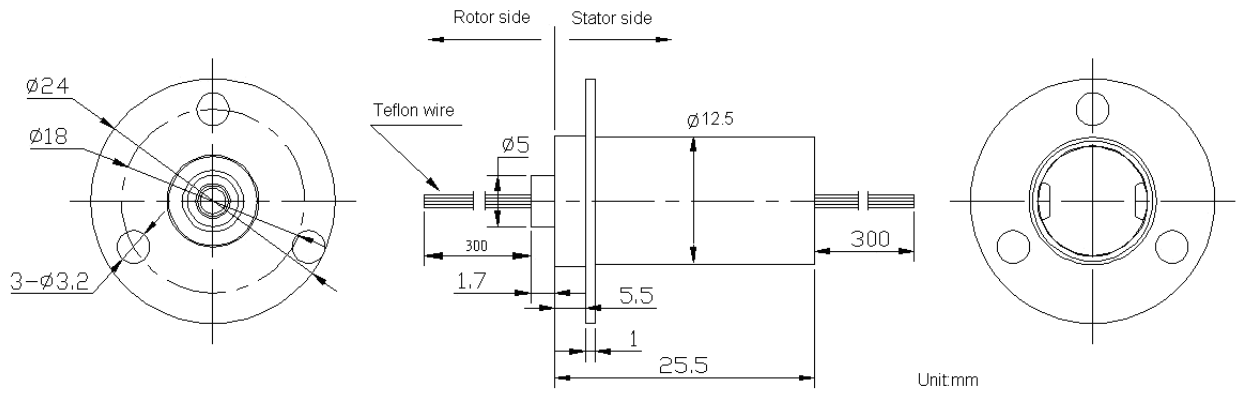
MODEL:BLC12-12A
